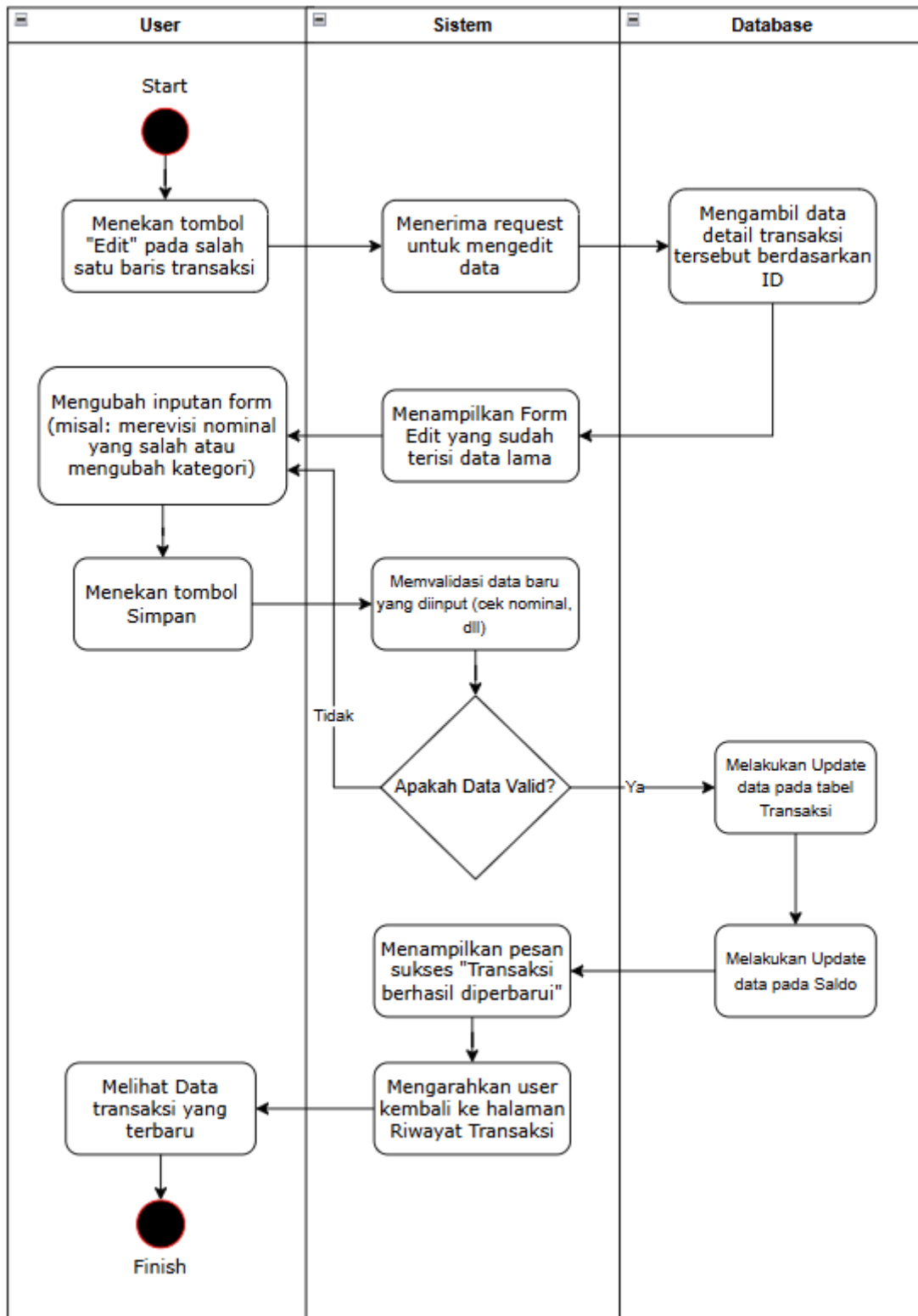
Gambar 8 Activity Diagram User Mengedit Data Transaksi
