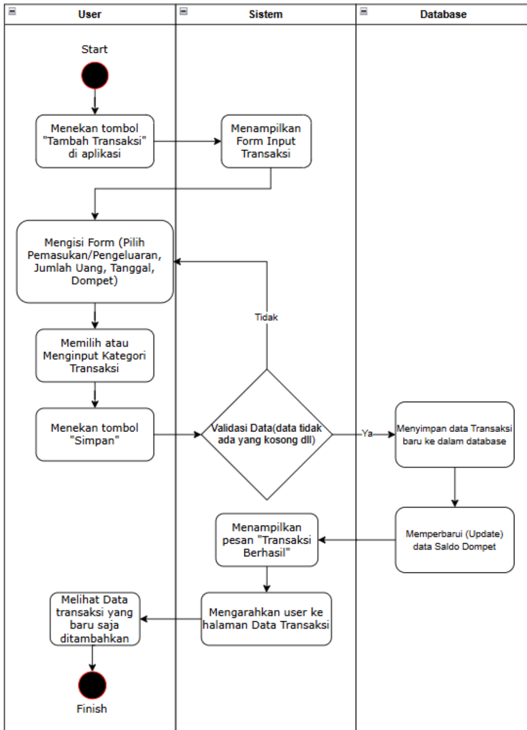
Gambar 6 Activity Diagram User Menginput Transaksi
