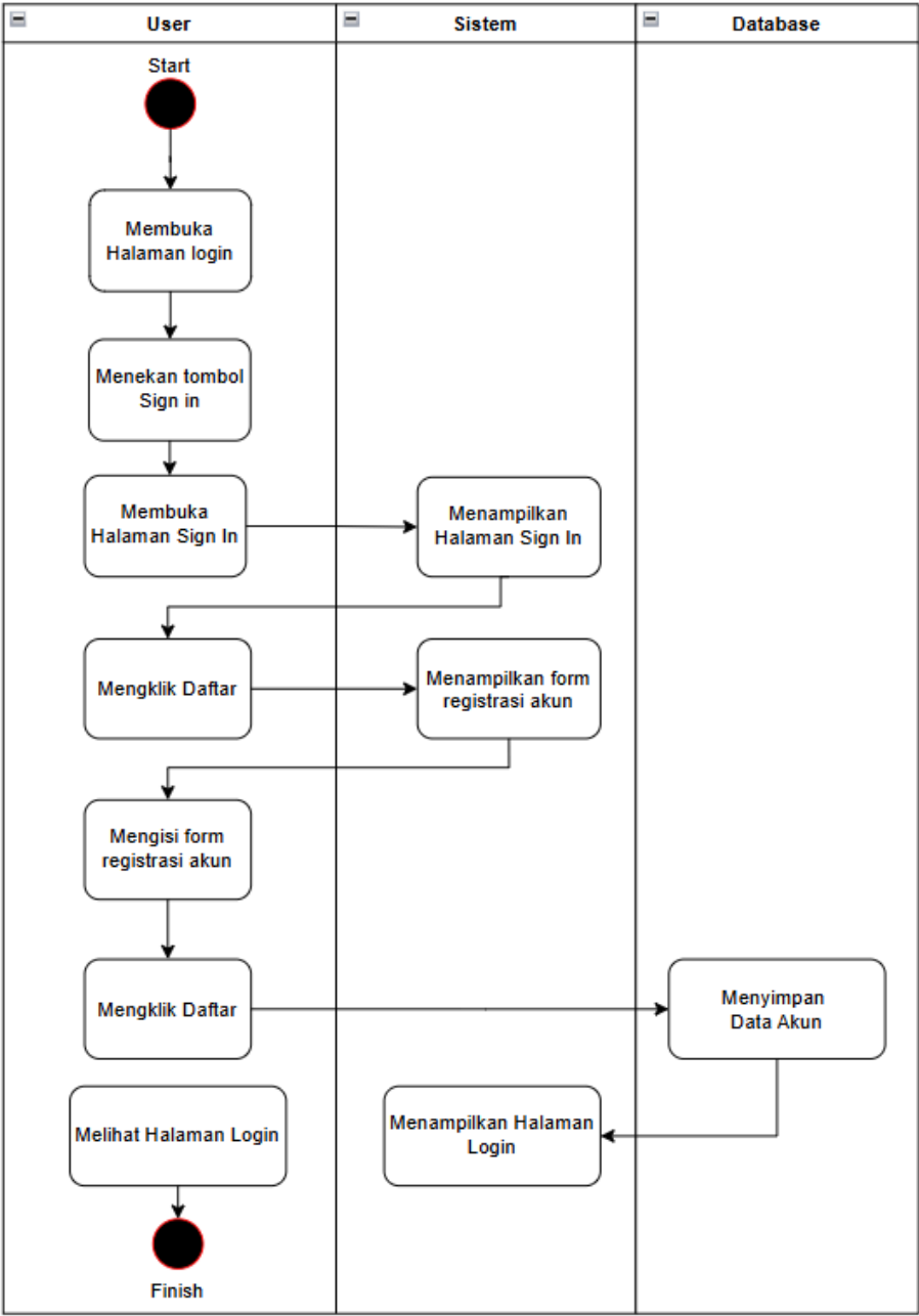
Gambar 2 Activity Diagram Registrasi User
