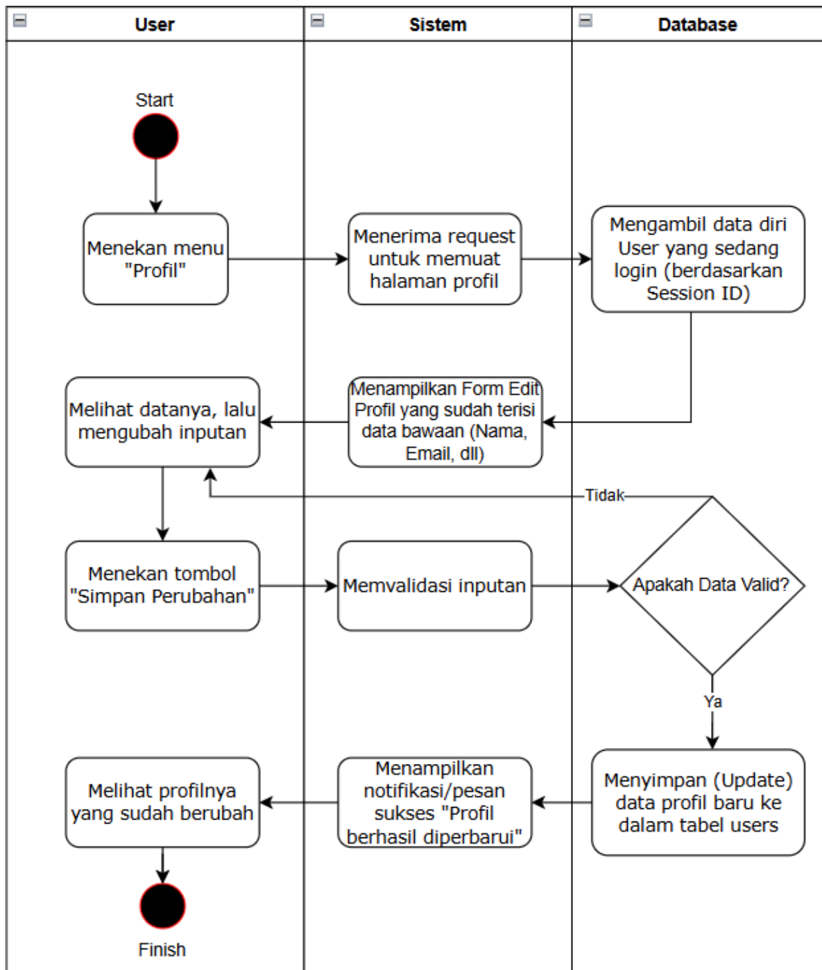
Gambar 4 Activity Diagram User Mengelola Profile User
