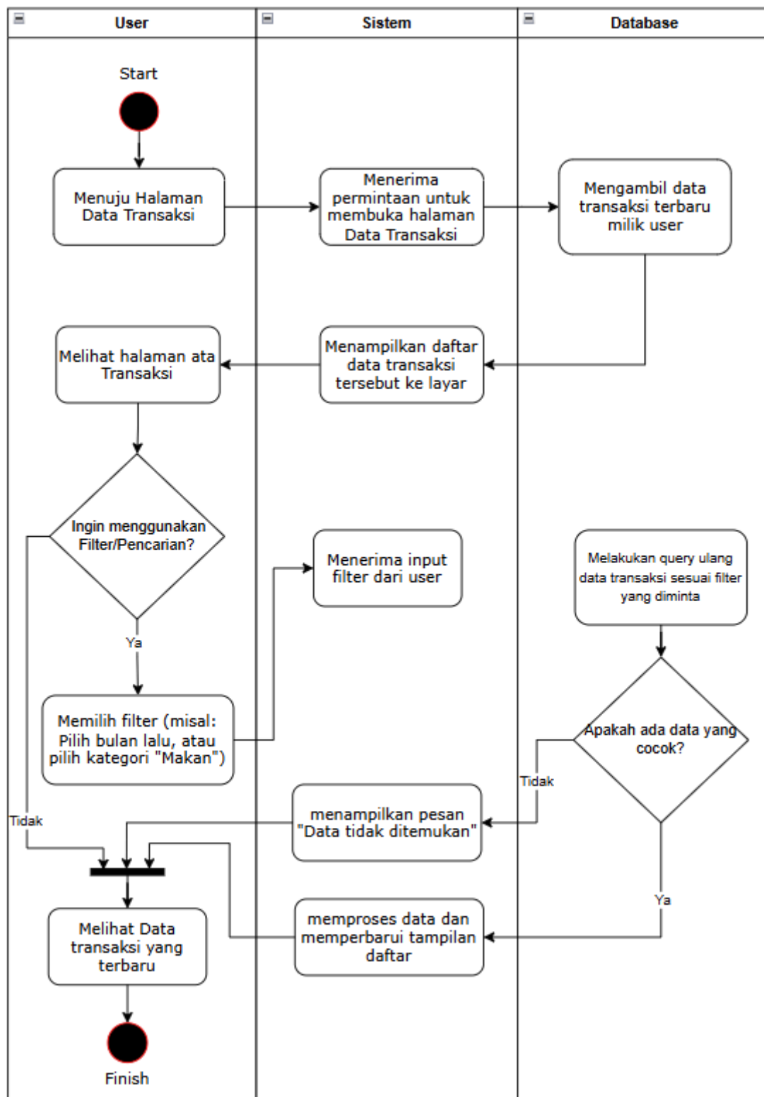
Gambar 7 Activity Diagram User Melihat Data Transaksi
