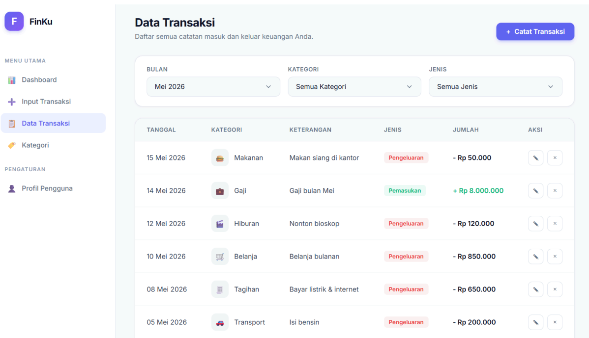
Gambar 28 System Prototype Data Transaksi User
