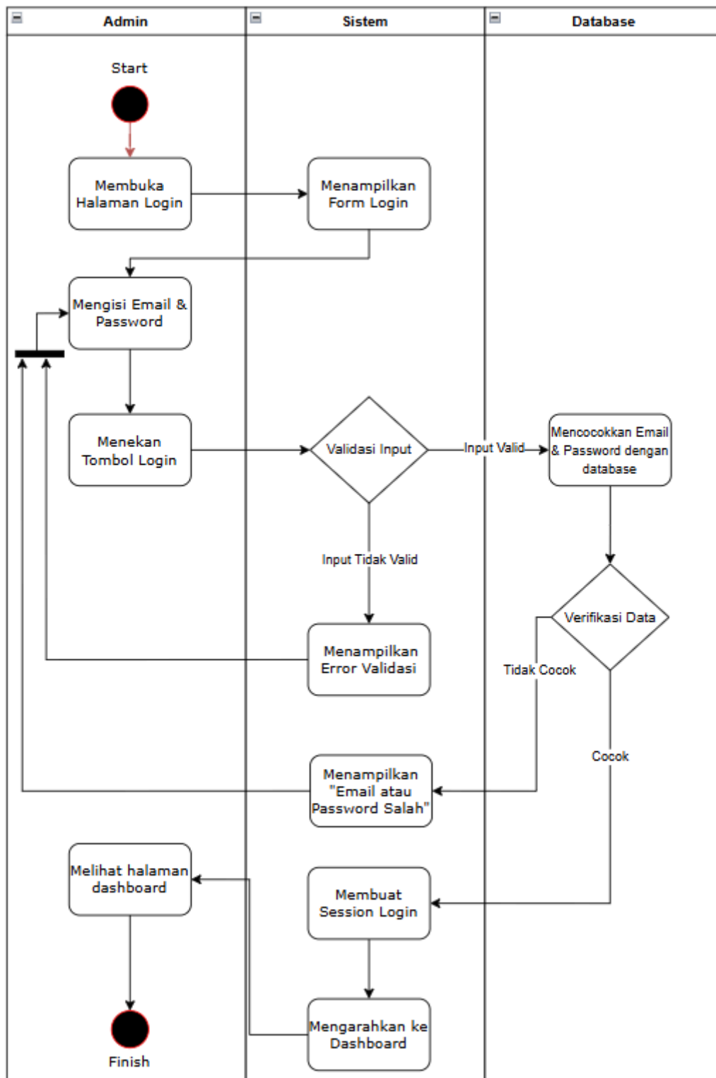
Gambar 10 Activity Diagram Login Admin
