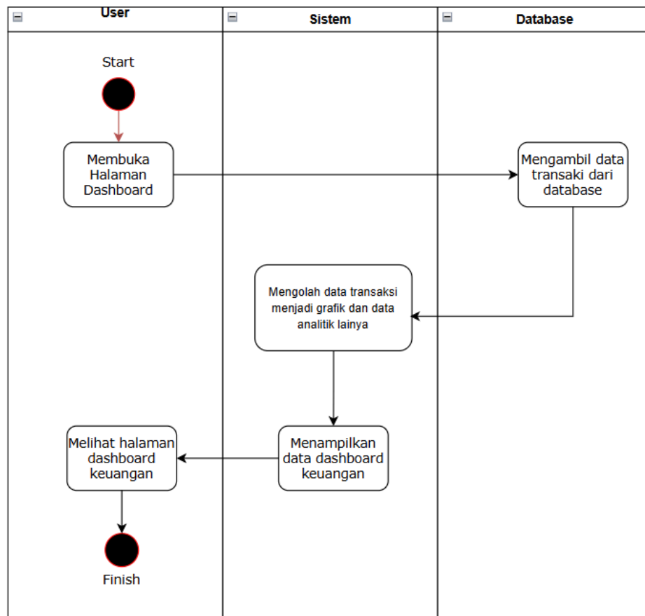
Gambar 5 Activity Diagram User Melihat Dashboard Keuangan
