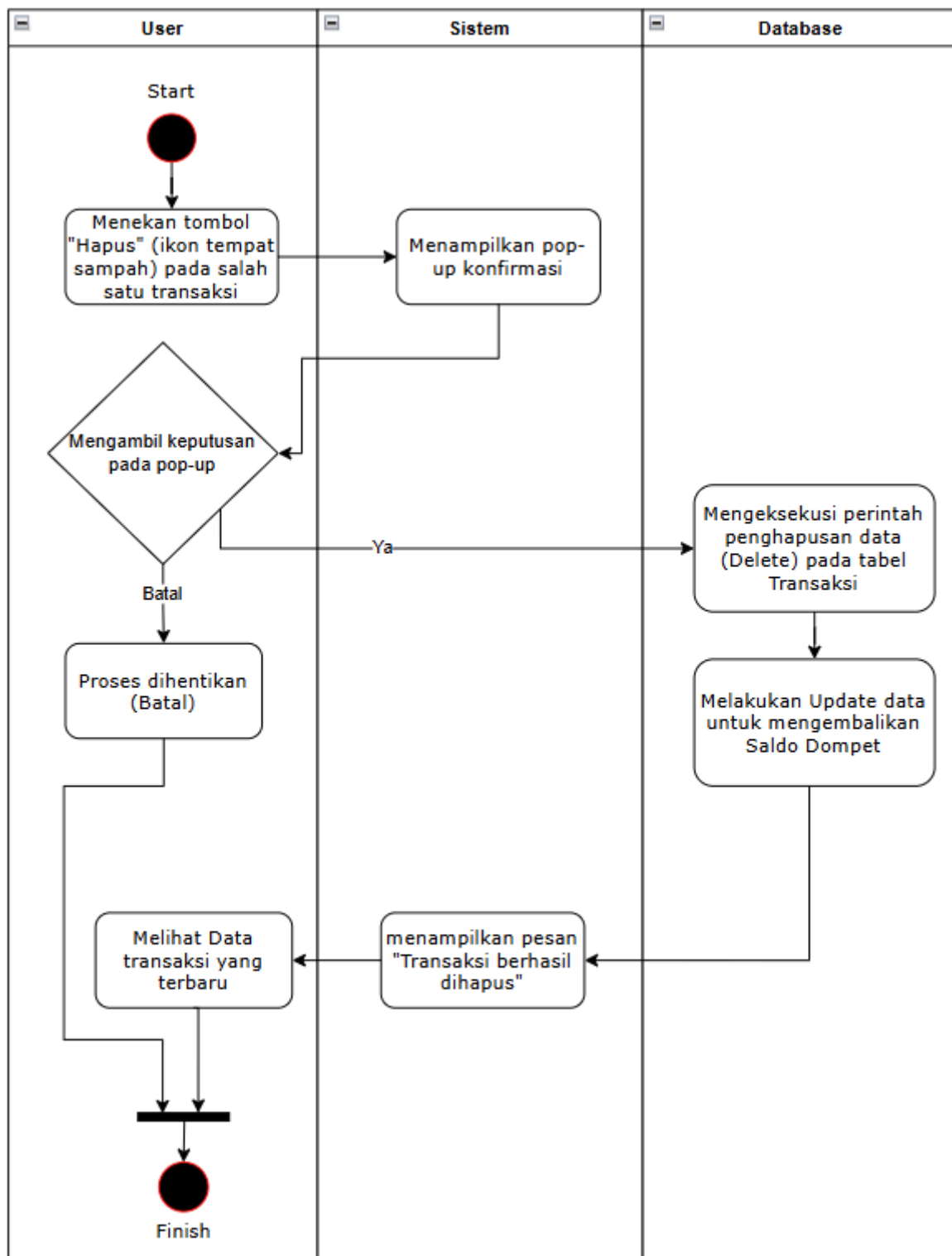
Gambar 9 Activity Diagram User Menghapus Data Transaksi
