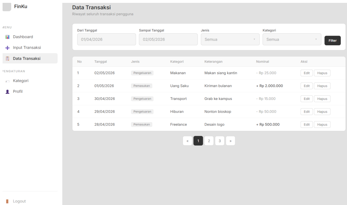
Gambar 17 UI Data Transaksi User
